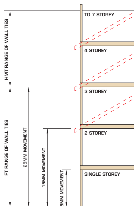
INTERMEDIATE FLOORS CONSTRUCTED USING EWP JOISTS
