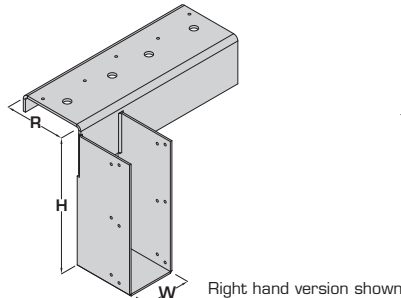
FMHIOR - OFFSET & RETURN
