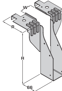
JHIR-W-H-R Example: JHIR-50-225-100 (Returns available to suit 100 & 140mm wide block work)
