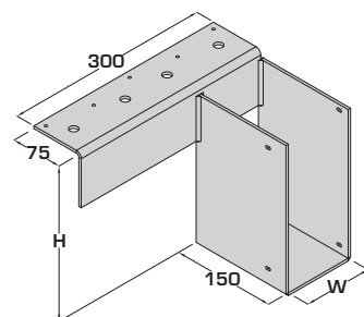
FTHIO-W-H-OFFSET DIRECTION Example: FTHIO-100-245-L FTHIO-100-245-R
