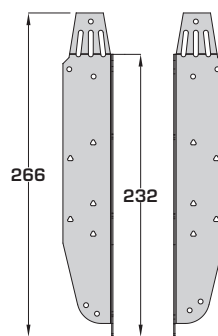
UH-235 (To suit 253 - 254mm deep open web joists)
