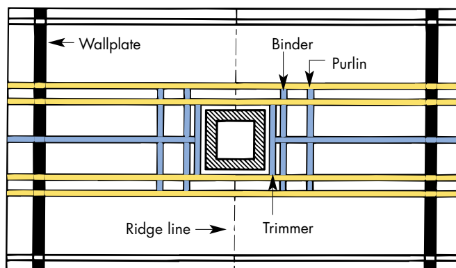
CHIMNEY DETAIL
